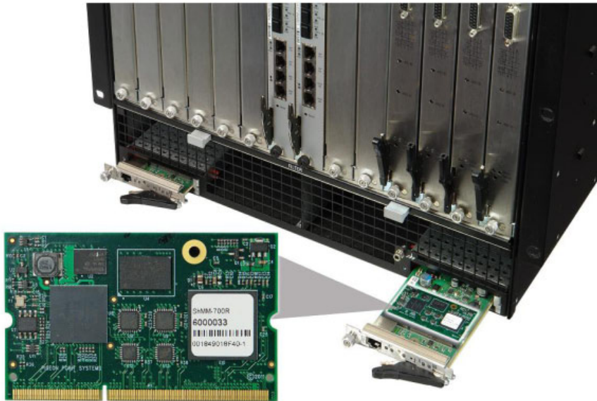
Image caption: Pigeon Point ShMM integrated in Schroff AdvancedTCA System
